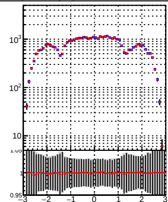
—•— DQM_TT_mkFit-DQM_lowptq_orig —•— DQM_TT_mkFit-DQM_lowptq_modi
