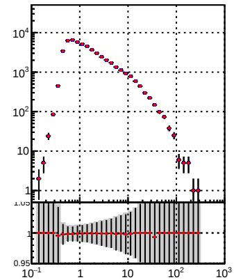
—•— DQM_TT_mkFit-DQM_lowptq_orig —•— DQM_TT_mkFit-DQM_lowptq_modi
