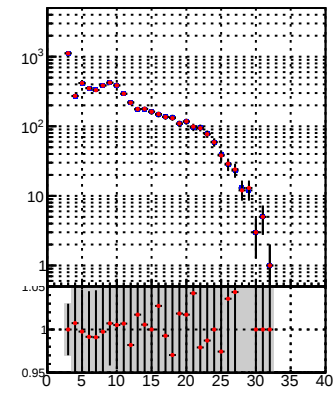
—•— DQM_TT_mkFit-DQM_lowptq_orig —•— DQM_TT_mkFit-DQM_lowptq_modi
