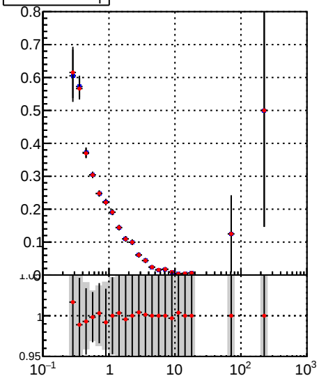
■ \text{DQM\_TT\_mkFit-DQM\_lowptq\_orig} ● \text{DQM\_TT\_mkFit-DQM\_lowptq\_modi}
