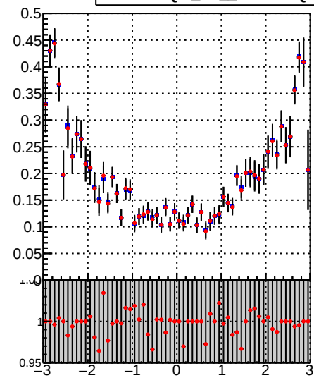
■ \text{DQM\_TT\_mkFit-DQM\_lowptq\_orig} ● \text{DQM\_TT\_mkFit-DQM\_lowptq\_modi}
