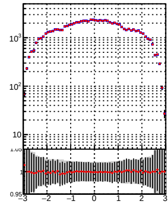
N of reco track vs \eta Legend: DQM_TT_mkFit-DQM_lowptq_orig (blue line with dots) DQM_TT_mkFit-DQM_lowptq_modi (red line with dots)
