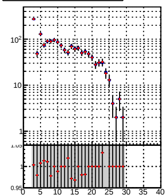
DQM_TT_mkFit-DQM_lowptq_orig DQM_TT_mkFit-DQM_lowptq_modi
