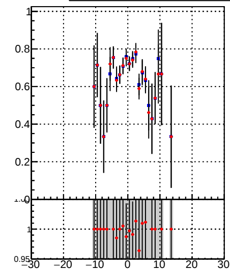
■ DQM_TT_mkFit-DQM_lowptq_orig ● DQM_TT_mkFit-DQM_lowptq_modi
