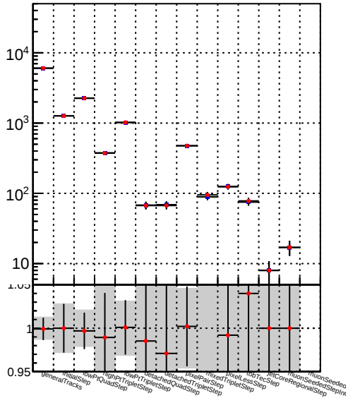
Number —●— DQM_TT_mkFit-DQM_lowptq_modi
