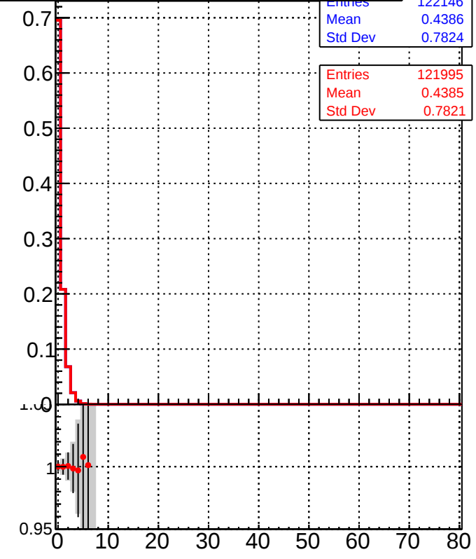
Legend: DQM_TT_mkFit-DQM_lowptq_orig (grey bars), DQM_TT_mkFit-DQM_lowptq_modi (red line with dots)
