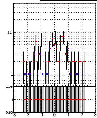
N of reco track vs \eta DQM TT mkFit-DQM_lowptq_orig N of reco track vs \eta DQM TT mkFit-DQM_lowptq_modi
