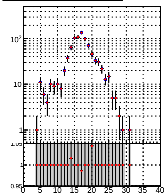
—•— DQM_TT mkFit-DQM_lowptq_orig —+— DQM_TT mkFit-DQM_lowptq_modi
