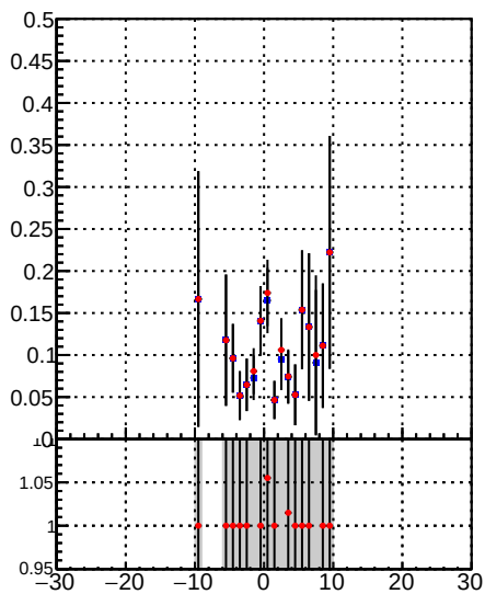
Fake rate vs d —•— DQM TT mkFit-DQM_lowptq_orig —•— DQM TT mkFit-DQM_lowptq_modi
