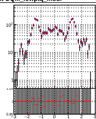
—●— DQM_TT_mkFit-DQM_lowptq_orig —●— DQM_TT_mkFit-DQM_lowptq_modi
