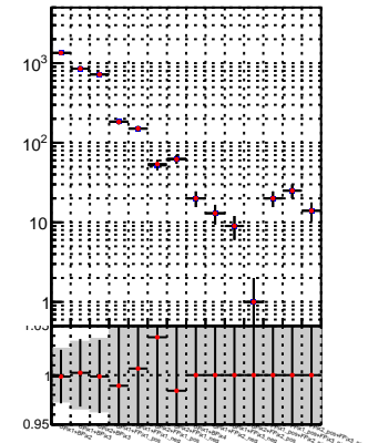
N of reco track vs. \chi^2 DQM_TT mkFit-DQM_lowptq_orig DQM_TT mkFit-DQM_lowptq_modi
