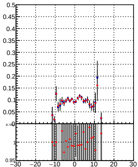
Fake rate vs d Legend: - DQM TT (blue dots) - mkFit-DQM_lowptq_orig (red dots)
