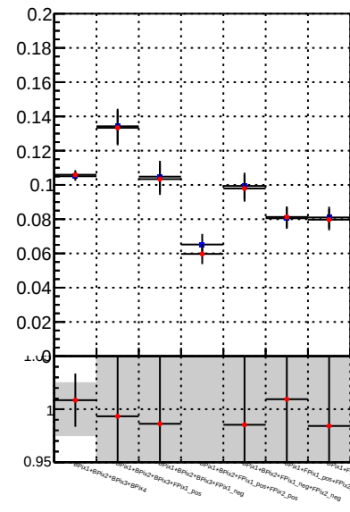
Fake rate vs. —•— DQM_TT_mkFit-DQM_lowptq_orig —•— DQM_TT_mkFit-DQM_lowptq_modi
