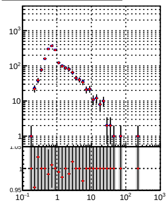
—•— DQM_TT_mkFit-DQM_lowptq_orig —•— DQM_TT_mkFit-DQM_lowptq_modi
