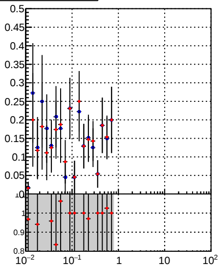
—•— DQM_TT_mkFit-DQM_lowptq_orig —•— DQM_TT_mkFit-DQM_lowptq_modi
