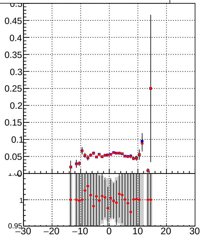
DQM_TT_mkFit-DQM_lowptq_orig DQM_TT_mkFit-DQM_lowptq_modi
