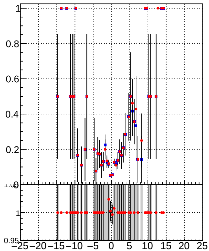
DQM_TT_mkFit-DQM_lowptq_orig DQM_TT_mkFit-DQM_lowptq_modi
