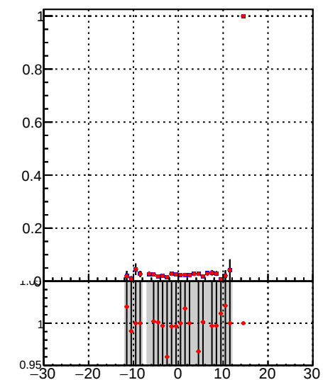
Fake rate vs d —•— DQM_TT_mkFit-DQM_lowptq_orig —•— DQM_TT_mkFit-DQM_lowptq_modi
