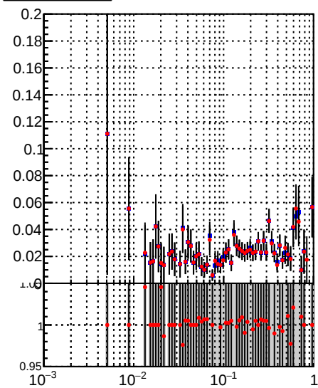
Fake rate vs \mu Legend: DQM_TT_mkFit-DQM_lowptq_orig (blue squares) DQM_TT_mkFit-DQM_lowptq_modi (red circles)
