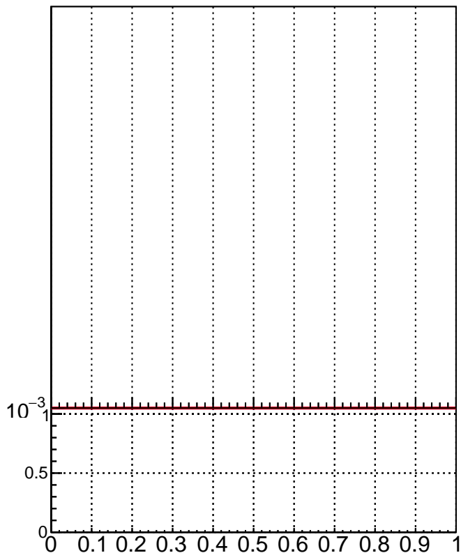
RecoPVAssoc2GenPVnotmatched_missing
