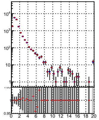
N of associated (recoSim) tracks vs. \chi^2
