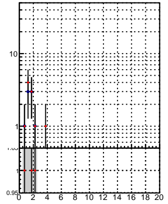
N of associated (recoSim) looper tracks vs. \chi^2
