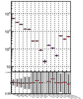
N of associated (recoSim) tracks vs. \chi^2
