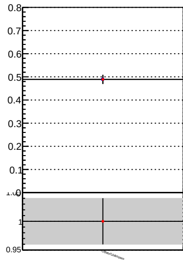
Fake rate vs. —•— DQM_TT_mkFit-DQM_lowptq_orig —•— DQM_TT_mkFit-DQM_lowptq_modi
