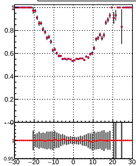
—•— DQM_TT_mkFit-DQM_lowptq_orig —•— DQM_TT_mkFit-DQM_lowptq_modi
