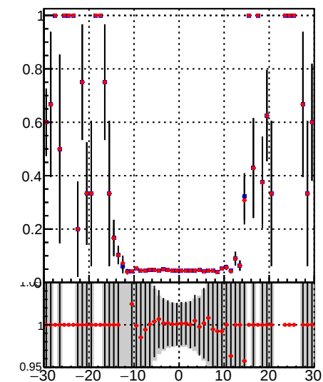
Fake rate vs d —•— DQM TT mkFit-DQM_lowptq_orig —•— DQM TT mkFit-DQM_lowptq_modi
