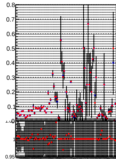
Fake rate vs. DQM_TT_mkFit-DQM_lowptq_orig DQM_TT_mkFit-DQM_lowptq_modi
