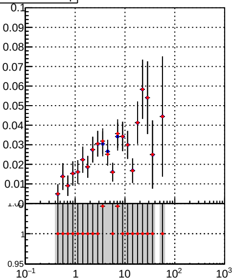
Legend: —■— DQM_TT_mkFit-DQM_lowptq_orig —●— DQM_TT_mkFit-DQM_lowptq_modi
