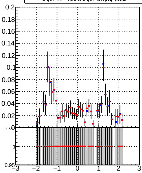
Legend: —■— DQM_TT_mkFit-DQM_lowptq_orig —●— DQM_TT_mkFit-DQM_lowptq_modi
