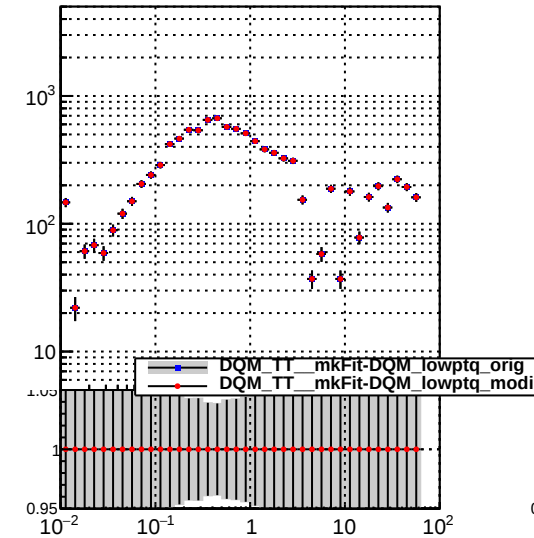
N of simulated tracks vs transverse vert position
