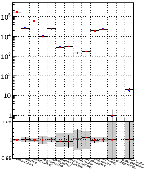
Number —●— DQM_TT_mkFit-DQM_lowptq_modi
