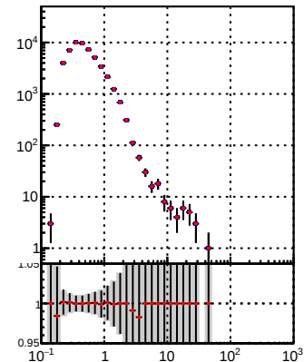
—•— DQM_TT_mkFit-DQM_lowptq_orig —•— DQM_TT_mkFit-DQM_lowptq_modi
