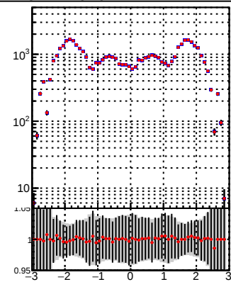
—•— DQM_TT_mkFit-DQM_lowptq_orig —•— DQM_TT_mkFit-DQM_lowptq_modi
