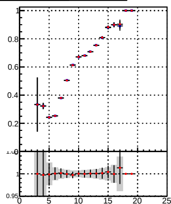
Fake rate vs hit Legend: DQM_TT_mkFit-DQM_lowptq_orig (blue line with dots), DQM_TT_mkFit-DQM_lowptq_modi (red line with dots)
