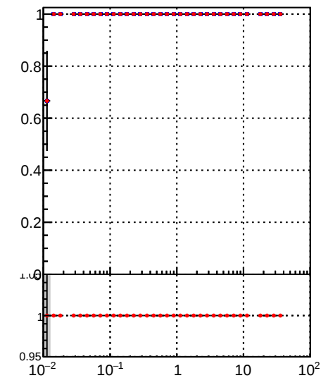
Fake rate vs vertpos Legend: DQM_TT_mkFit-DQM_lowptq_orig (grey line with error bars) DQM_TT_mkFit-DQM_lowptq_modi (red line with error bars)
