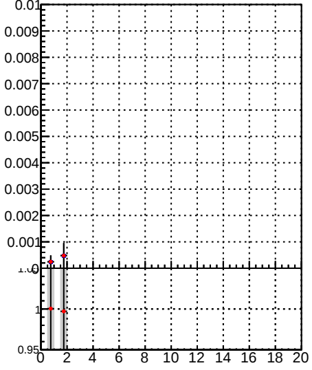
Fake rate vs. —●— DQM TT mkFit-DQM_lowptq_orig —●— DQM TT mkFit-DQM_lowptq_modi
