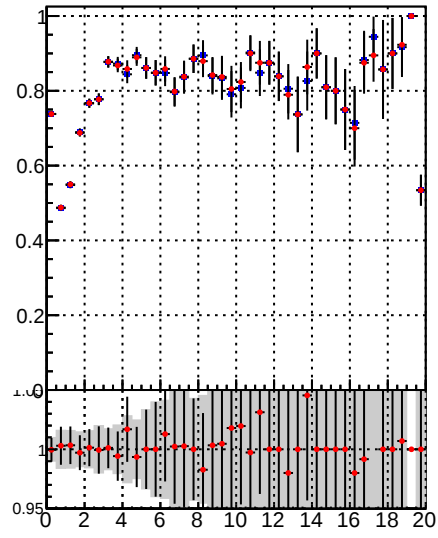
Fake rate vs. —●— DQM TT mkFit-DQM_lowptq_orig —●— DQM TT mkFit-DQM_lowptq_modi
