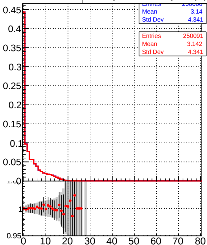
Legend: DQM_TT_mkFit-DQM_lowptq_orig (Gray shaded area) DQM_TT_mkFit-DQM_lowptq_modi (Red line with markers)
