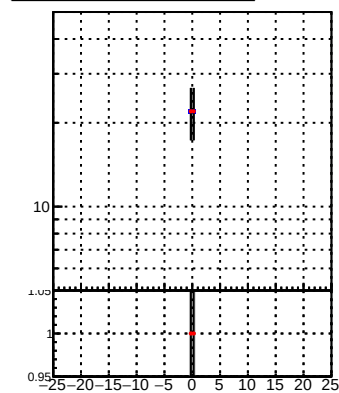
N of associated (recoToSim) loopers tracks vs dxy(PV)
