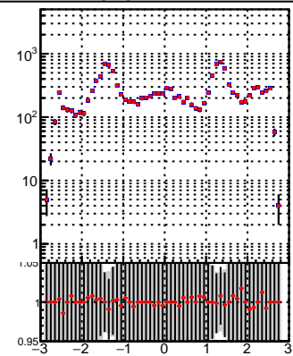
N of reco track vs \eta vs \phi —•— DQM_TT_mkFit-DQM_lowptq_orig —•— DQM_TT_mkFit-DQM_lowptq_modi
