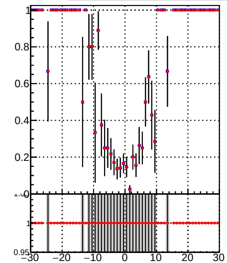
DQM_TT_mkFit-DQM_lowptq_orig DQM_TT_mkFit-DQM_lowptq_modi
