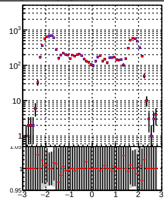
N of reco track vs \eta DQM TT mkFit-DQM_lowptq_orig DQM TT mkFit-DQM_lowptq_modi
