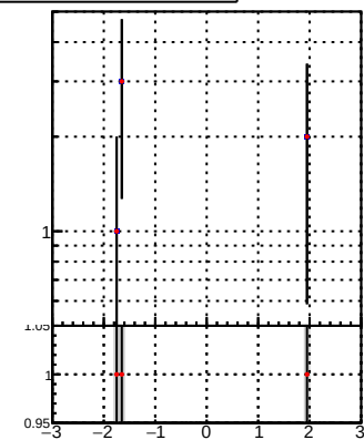
N of associated (recoToSim) tracks vs \eta DQM TT mkFit-DQM_lowptq_orig DQM TT mkFit-DQM_lowptq_modi
