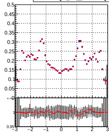
—•— DQM_TT_mkFit-DQM_lowptq_orig —•— DQM_TT_mkFit-DQM_lowptq_modi
