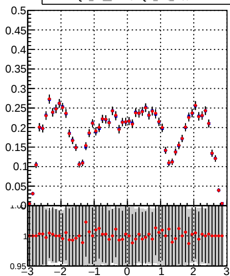
— DQM_TT_mkFit-DQM_init_orig — DQM_TT_mkFit-DQM_init_mod
