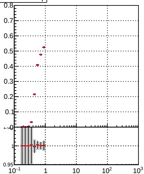
— DQM_TT_mkFit-DQM_init_orig — DQM_TT_mkFit-DQM_init_mod
