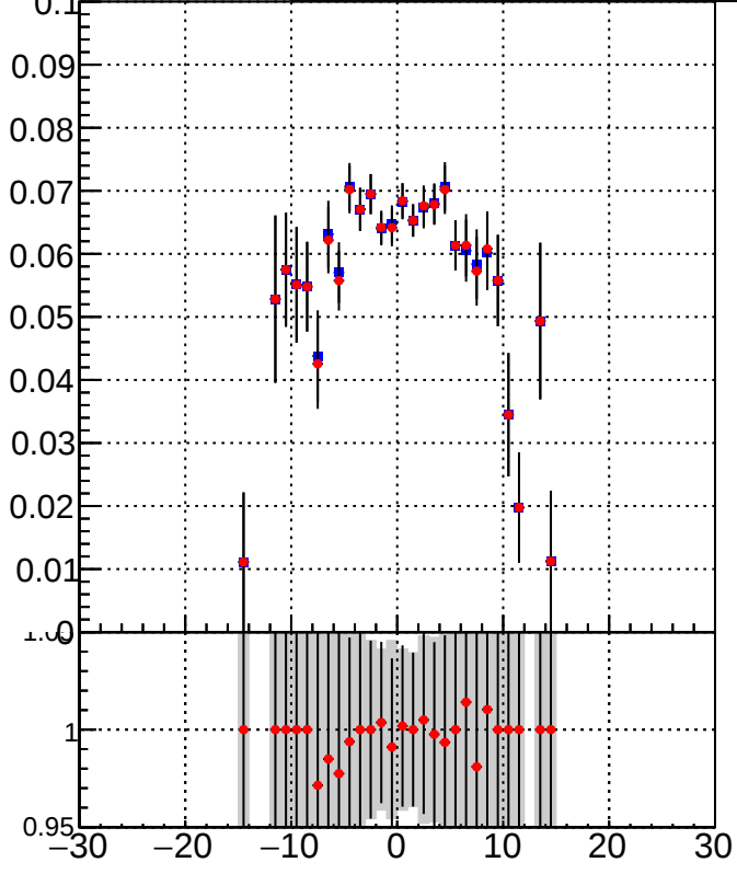
Efficiency vs Dz DQM_TT_mkFit-DQM_init_orig DQM_TT_mkFit-DQM_init_mod
