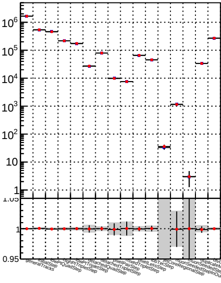
Number of pileup tracks vs collection
