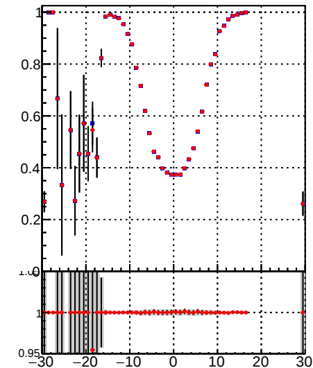
—•— DQM_TT_mkFit-DQM_init_orig —•— DQM_TT_mkFit-DQM_init_mod
