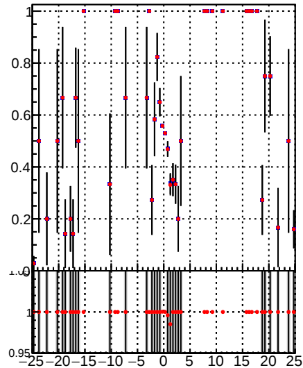
—•— DQM_TT_mkFit-DQM_init_orig —•— DQM_TT_mkFit-DQM_init_mod
