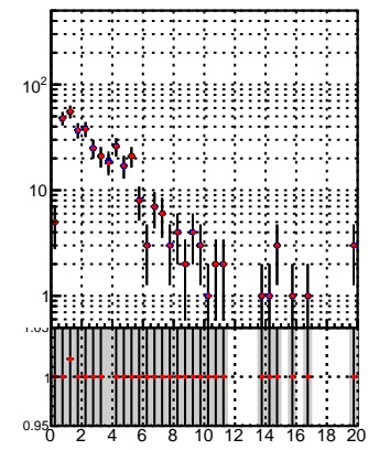
N of reco track vs. \chi^2 (with legend)
