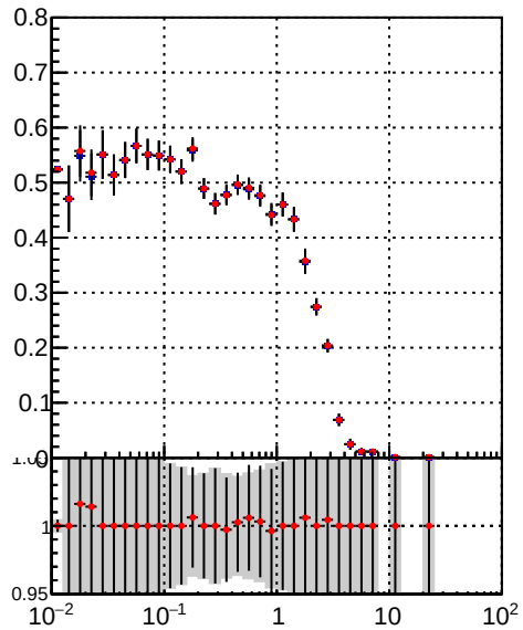
Efficiency vs. vertpos Legend: DQM_TT_mkFit-DQM_init_orig (blue line with error bars) DQM_TT_mkFit-DQM_init_mod (red line with error bars)
