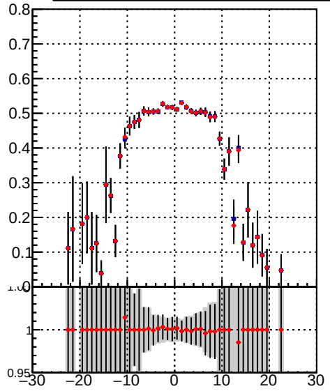
Efficiency vs. vertpos Legend: DQM_TT_mkFit-DQM_init_orig (blue line with error bars) DQM_TT_mkFit-DQM_init_mod (red line with error bars)
