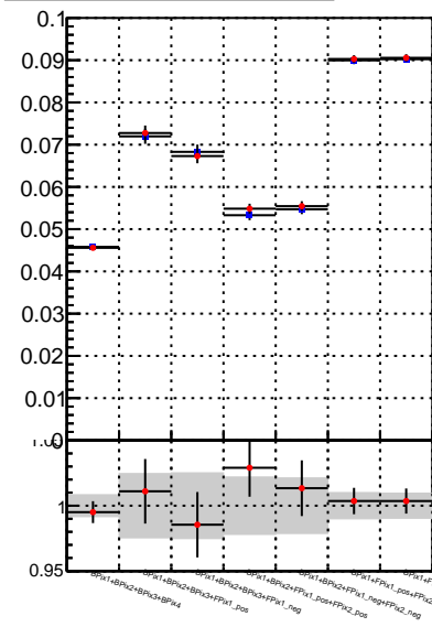
Fake rate vs. —•— DQM_TT_mkFit-DQM_init_orig —•— DQM_TT_mkFit-DQM_init_mod
