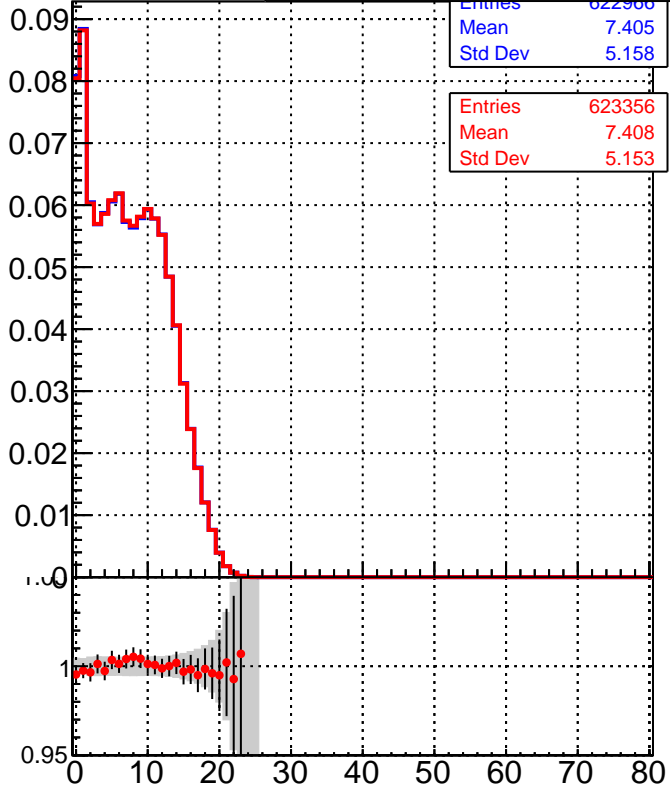
—■— DQM_TT_mkFit-DQM_init_orig —●— DQM_TT_mkFit-DQM_init_mod
