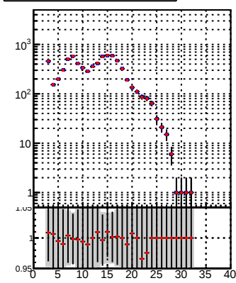
DQM_TT_mkFit-DQM_init_orig DQM_TT_mkFit-DQM_init_mod
