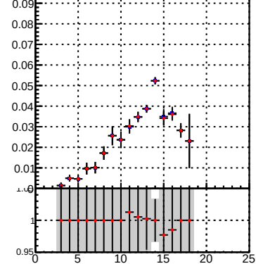
Efficiency vs pixel layer
