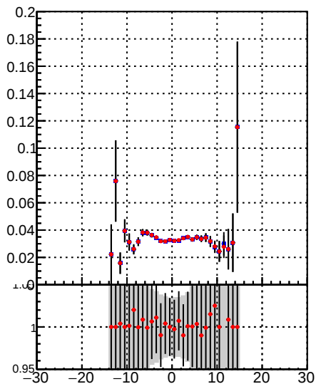
—●— DQM_TT_mkFit-DQM_init_orig —●— DQM_TT_mkFit-DQM_init_mod
